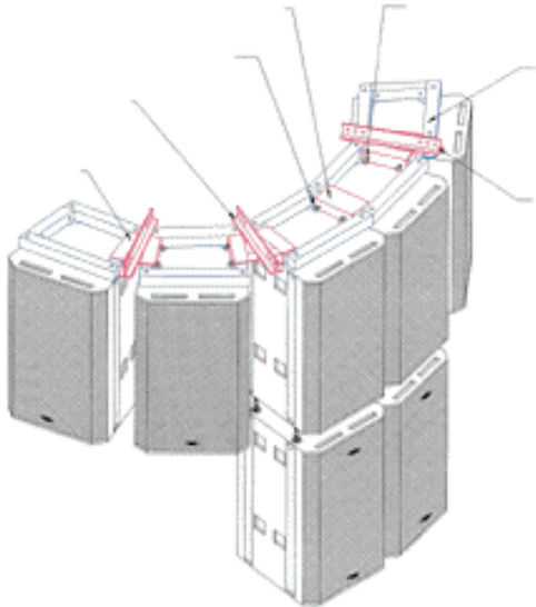
Apogee 3X3S2 Array with MARS Rigging
